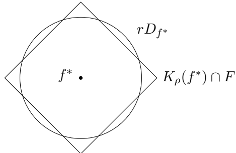
Figure 1: Localization of the set F \cap K_\rho(f^*) , i.e. its intersection with L_2(\mu) -balls of various radii r for the right choice of radius \rho , plays a central role in the analysis of the quadratic and multiplier processes.
