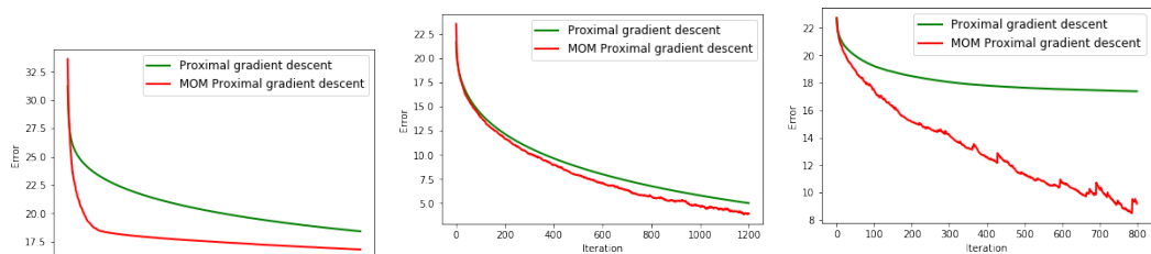
(a) Gaussian design and Gaussian noise. (b) Heavy-tailed noise \zeta (Student distribution of order 2) and standard Gaussian design. (c) Gaussian noise and heavy-tailed design (Student distribution of order 2).
